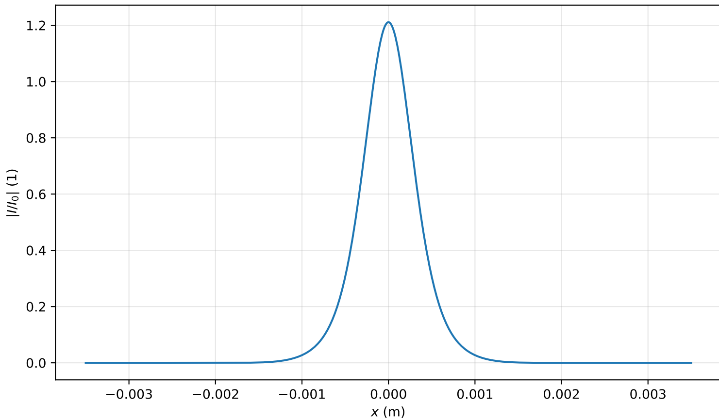
Intensity profile I(x, y = 0, z = 1.274m)/I_0 , P_{in}=0.7P_{cr} , artificial time
